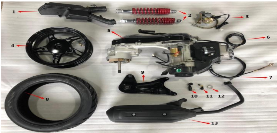
Figure B: rear shock,muffler,etc(图B: 后减震、消音器等)
