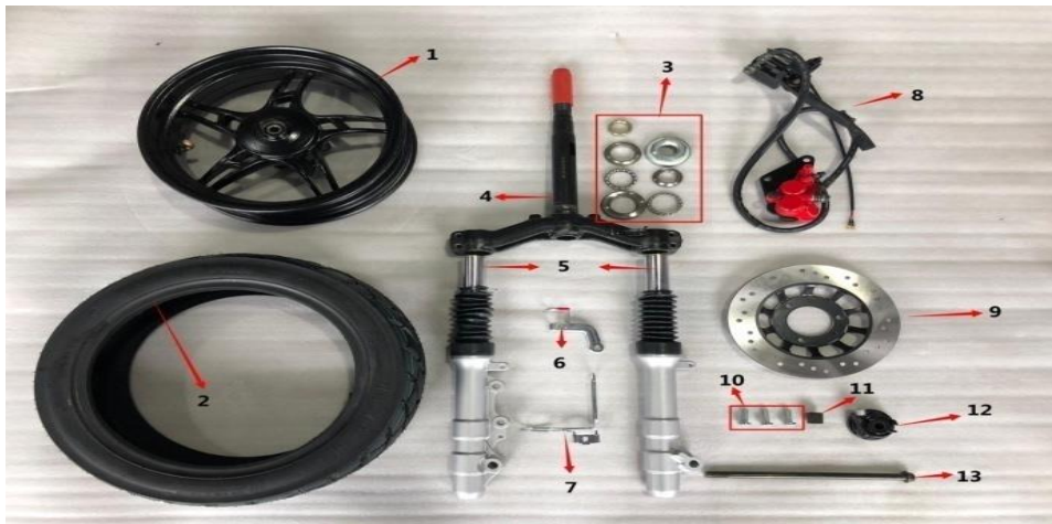
Figure C: front wheel, front shock, etc (图C: 前轮、前减震等)
