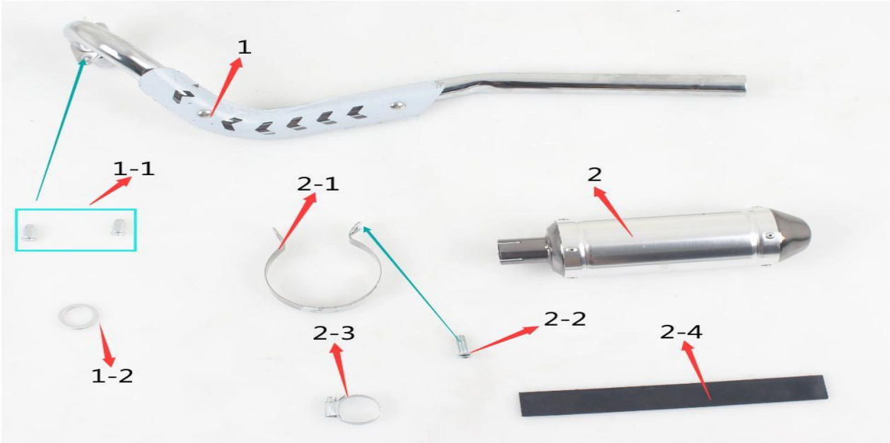
Figure A: the muffler components, oxygen sensor
