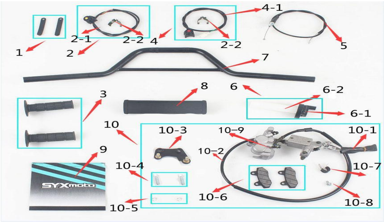
Figure B:Steering handle assembly, etc
