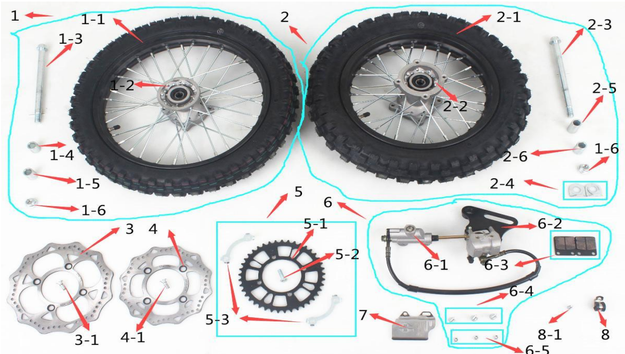
Figure L: front tires, rims, front drum brake, front disc brake etc.
