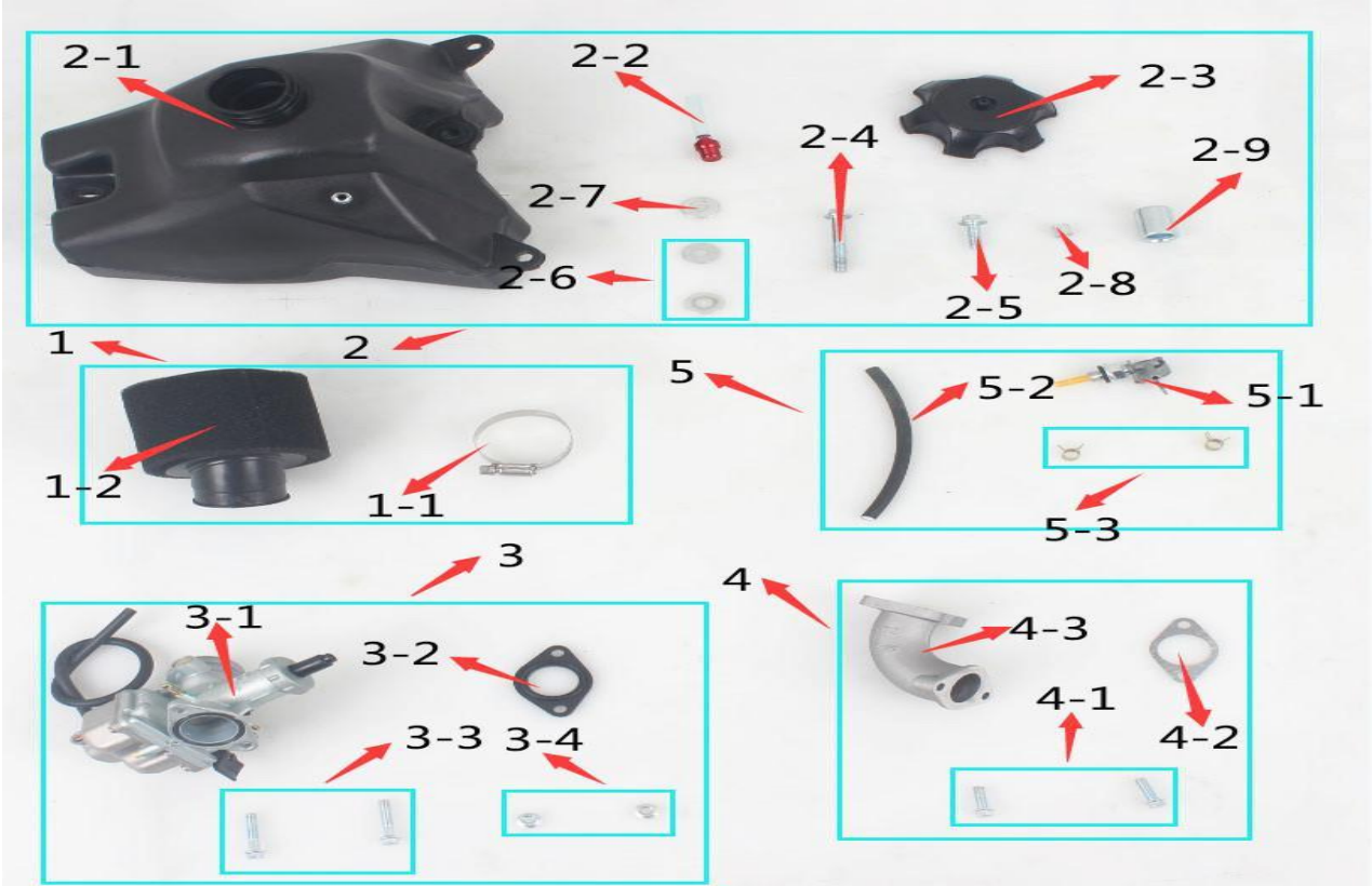
Figure F: the cushion, oil tank, tubing, etc.
