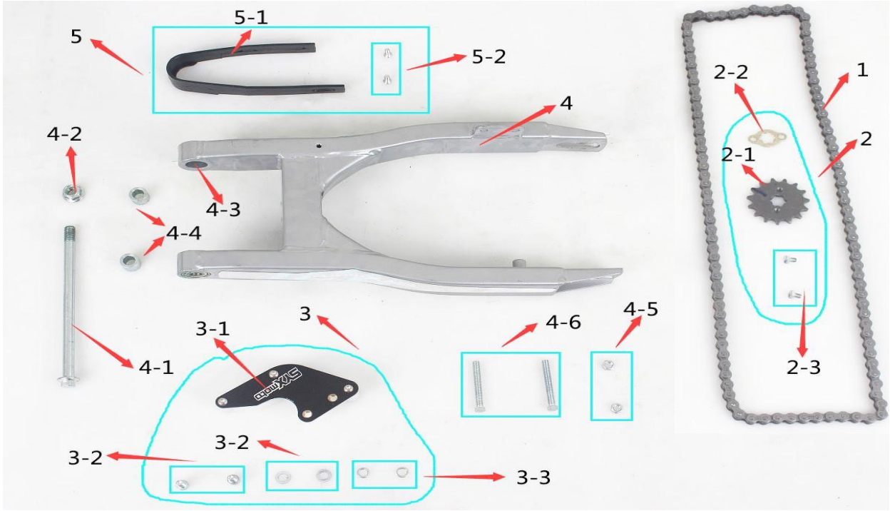
Figure D: rear fork components, brake components, etc.
