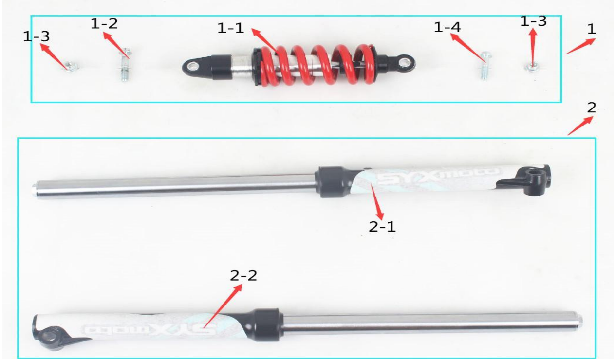
Figure C: Front shock absorption and rear shock absorption components
