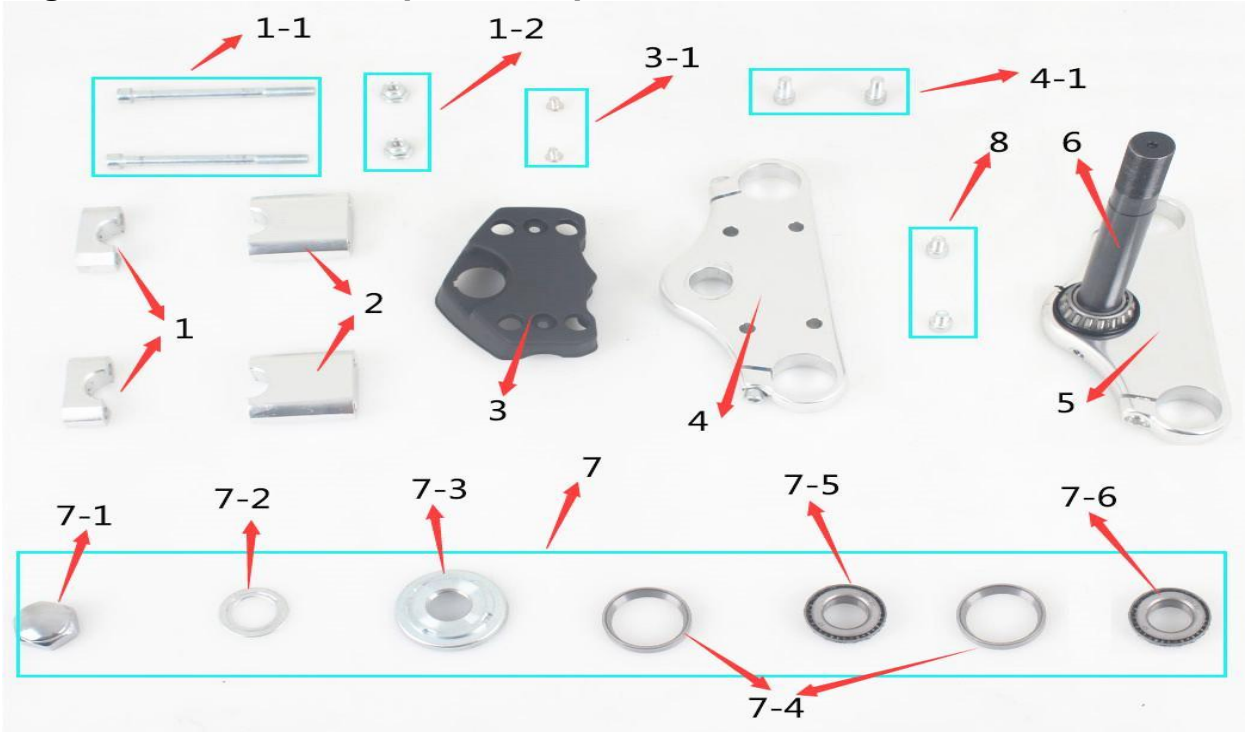
Figure J: shock, lower plate component, reflection lens, etc
